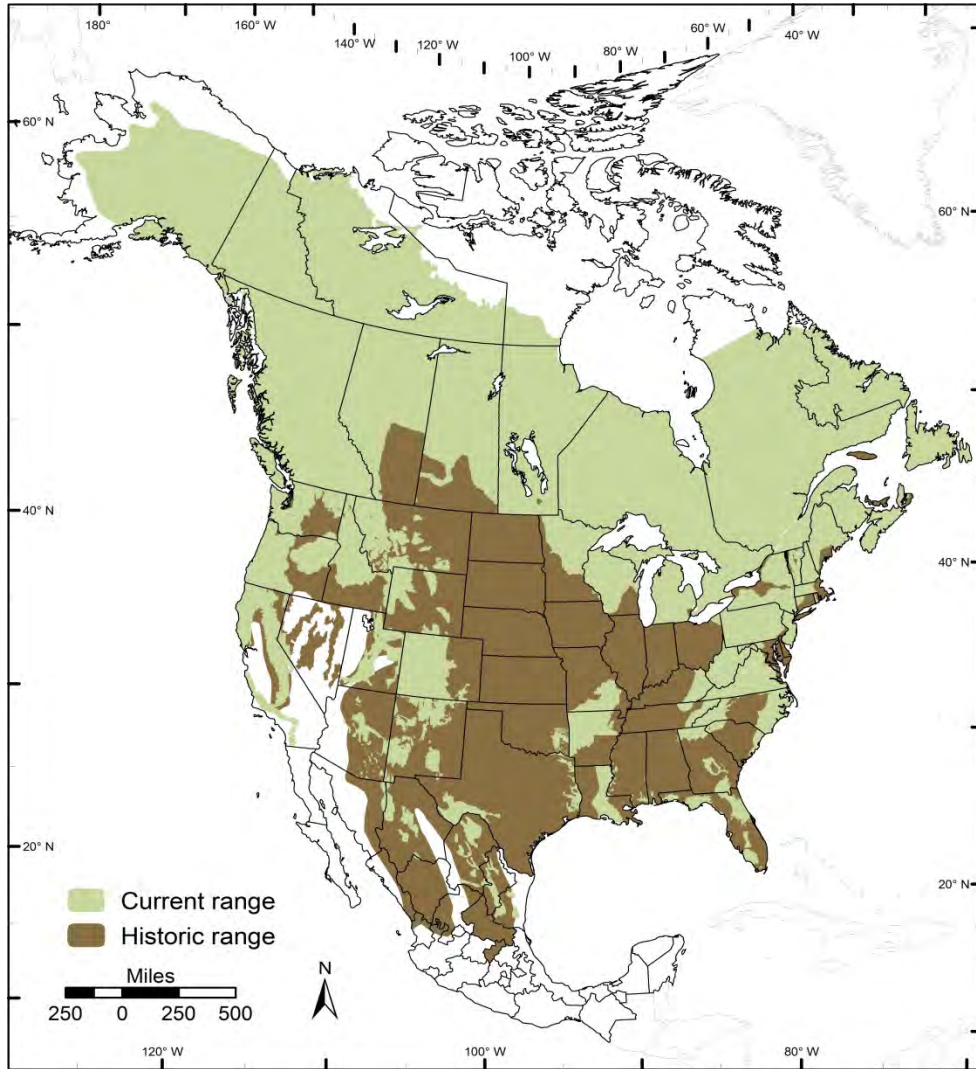
Figure 3. American black bear ( Ursus americanus ) historical and current range. From Garshelis et al. (2016), the IUCN Red list of threatened species.
